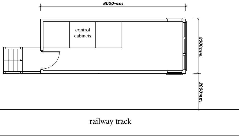
Ground Plan
